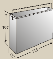
Stove Canopy with Top Flue Outlet
